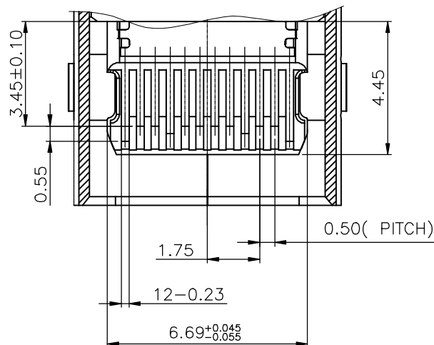
SECTION B-B
